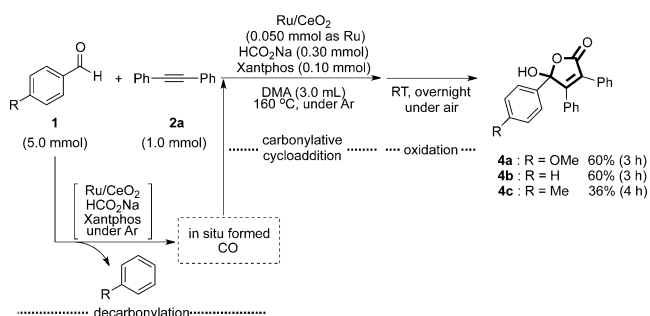
Scheme 4. [2+2+1] carbonylative cycloaddition of aldehydes and alkynes without using external CO.
