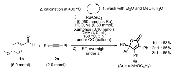
Scheme 6. Recycling of Ru/CeO 2 catalyst.
