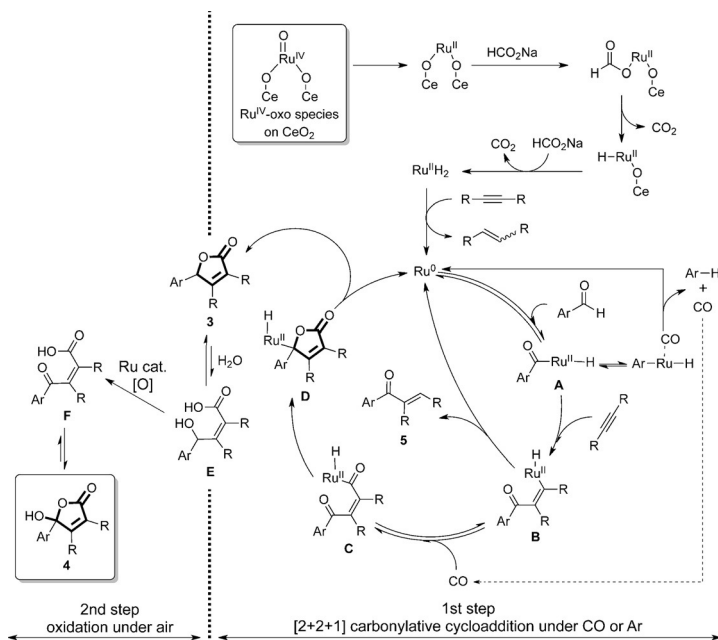
Scheme 5. Possible reaction route to \gamma -hydroxybutenolides.
