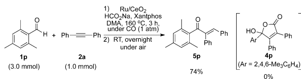
Scheme 3. Hydroacylation of the internal alkyne 2a with 1p by Ru/CeO 2 . DMA = N,N -dimethylacetamide.
