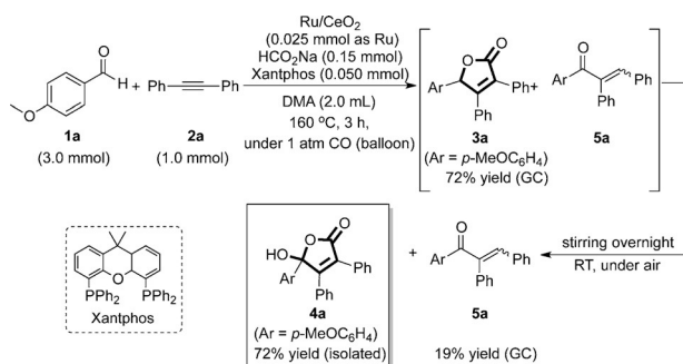
Scheme 2. Synthesis of the \gamma -hydroxybutenolide 4a by the [2+2+1] carbonylative cycloaddition of an aldehyde and alkyne, with subsequent oxidation by Ru/CeO 2 .
